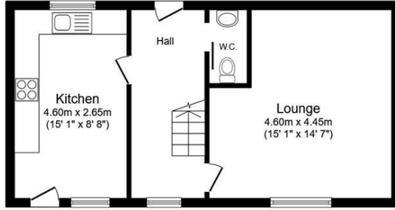
Ground Floor Floor area 42.3 sq.m. (455 sq.ft.)
